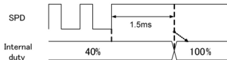
Figure 8.7 When "H" is held for 1.5ms or more from the last rising edge
