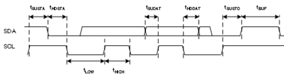
Figure 11.1 Electrical characteristics of I 2 C timing chart
