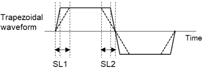
Fig. 4-19 Trapezoidal wave motor current rising / falling slope setting
