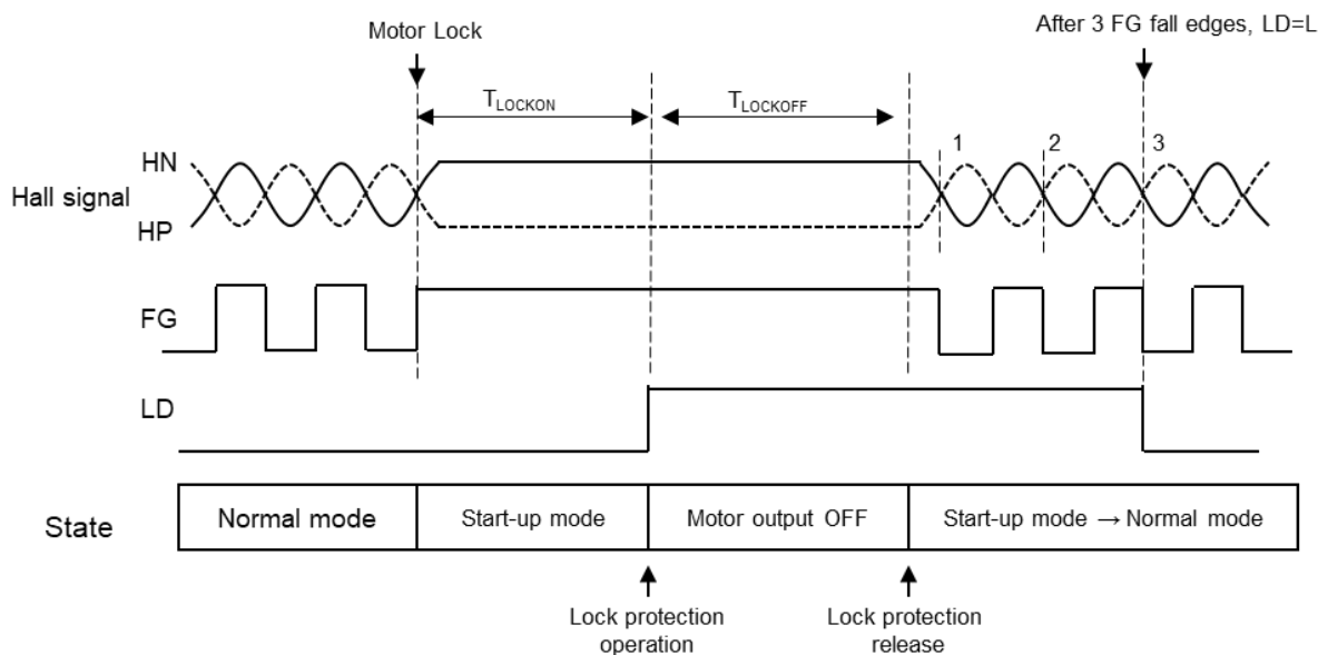
Fig. 4-7 Lock Protection Time for Detection and Release
