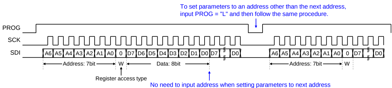
Fig.4-34 Register setting parameter setting command
