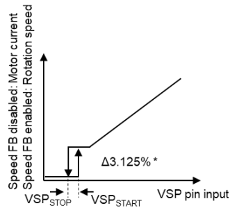
Fig 4-16 VSP at start and stop setting
