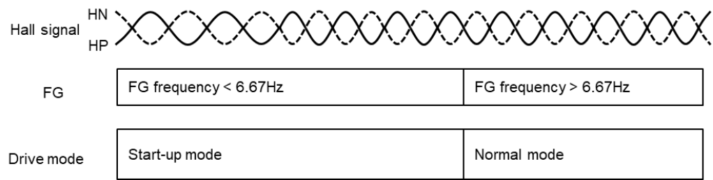
Fig. 4-3 Start-up mode / Normal mode switching
