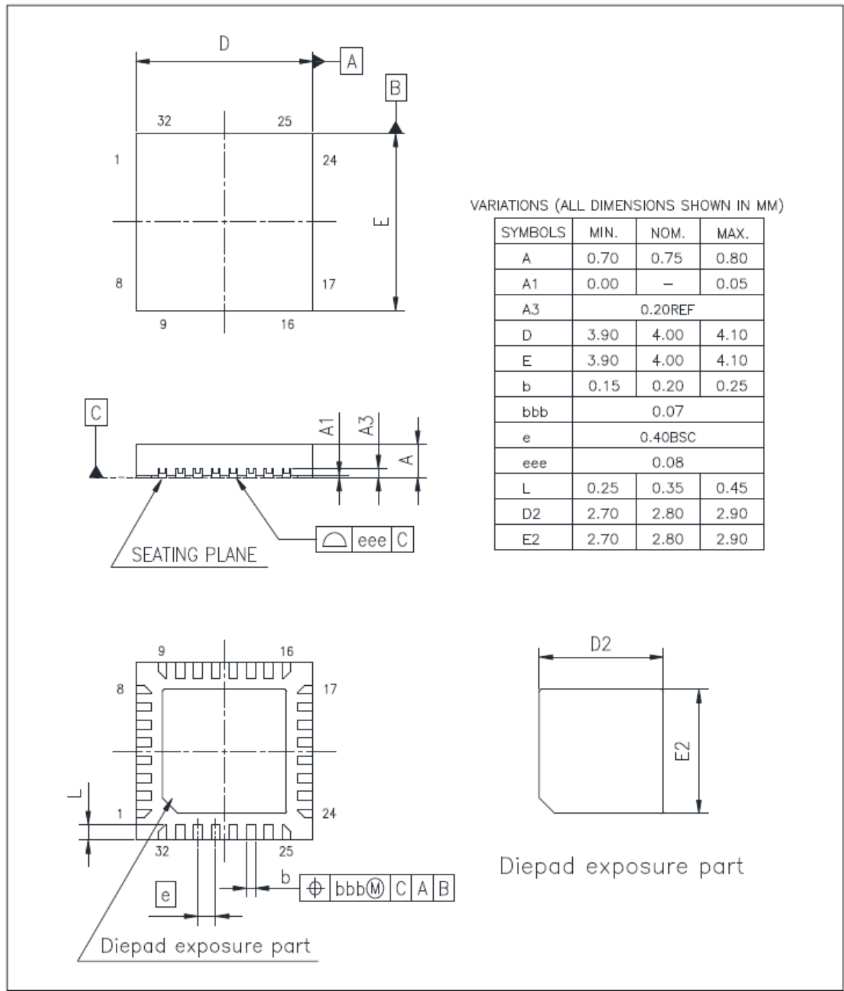
Fig. 5-1 Outline Drawing of package
