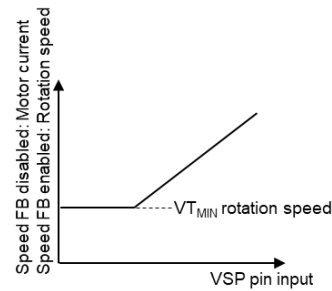
Fig 4-17 When not stop is selected in stop VSP setting
